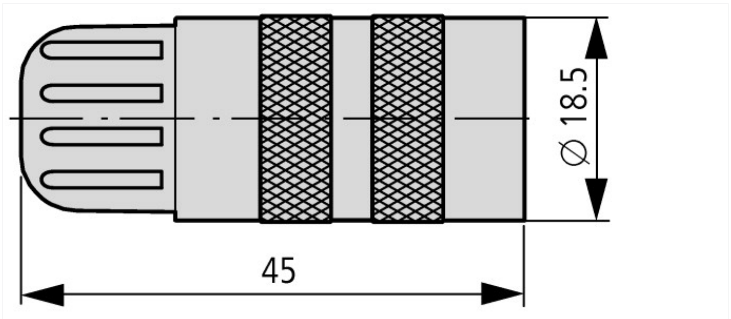
Plug connectors for SmartWire-DT round cables, flat
